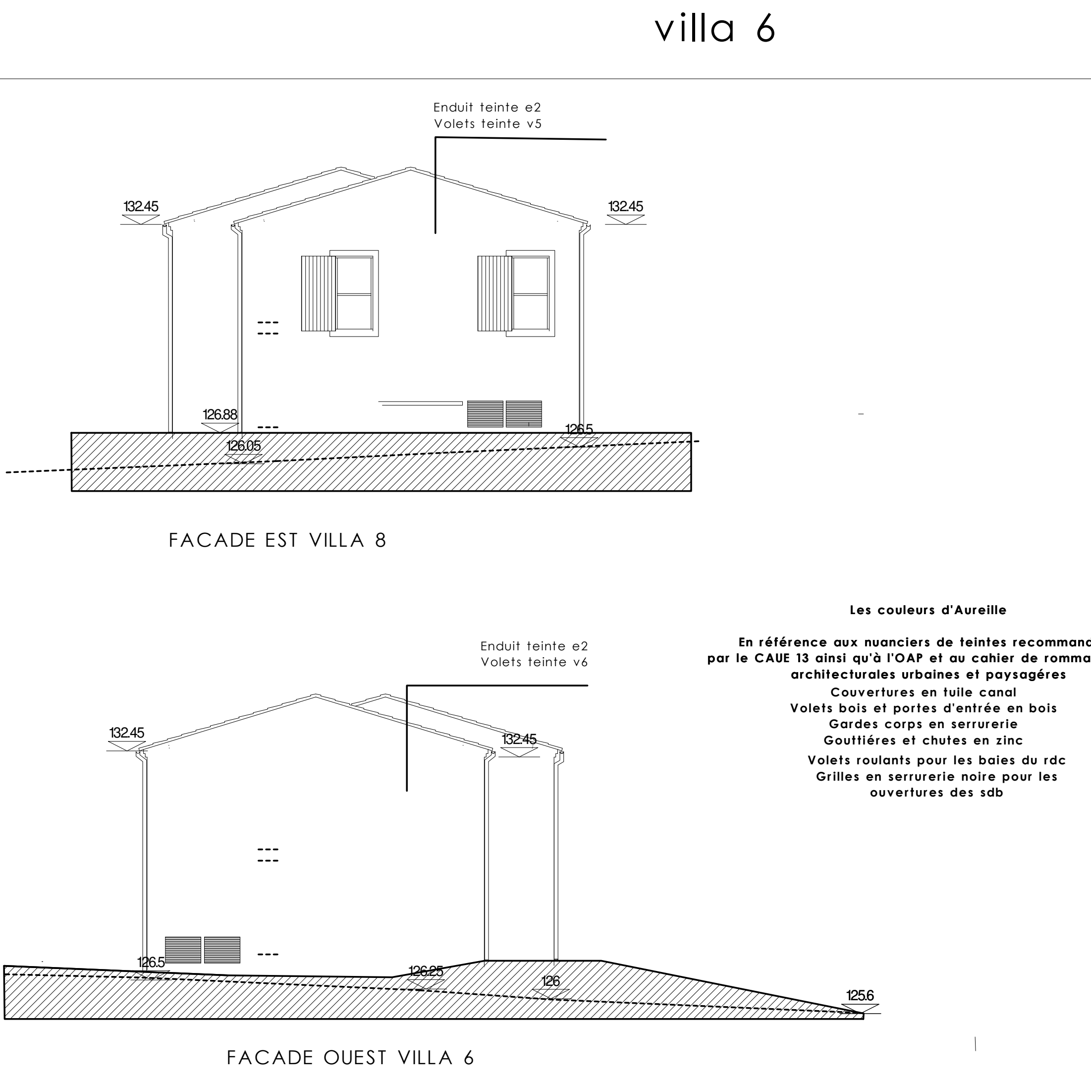
FACADES /100
